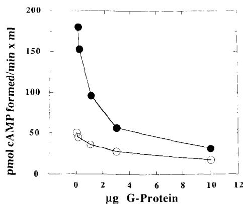
Fig. 3. The effect of G_o/G_i on G_s stimulated adenylate cyclase in dimyristoylphosphatidyl choline. Forskolin affinity purified cyclase was reconstituted with G_s and the indicated concentrations of G_o/G_i , and assayed in the presence (closed symbols) or absence (open symbols) of 10 \mu M GppNHp.
